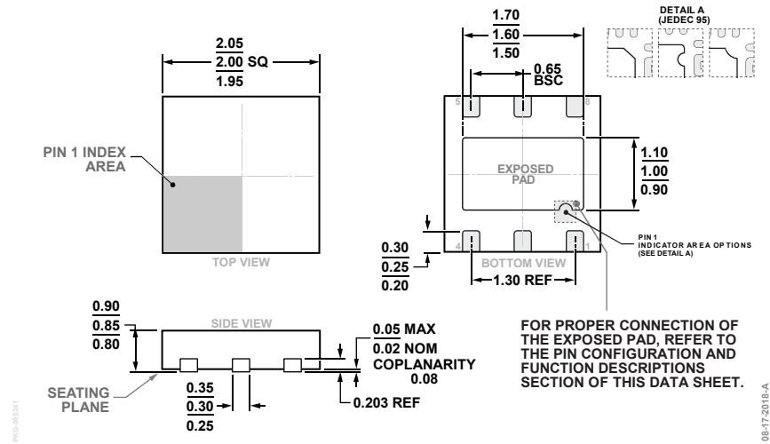
Figure 76. 6-Lead Lead Frame Chip Scale Package [LFCSP] 2 mm x 2 mm Body and 0.85 mm Package Height (CP-6-12) Dimensions shown in millimeters
