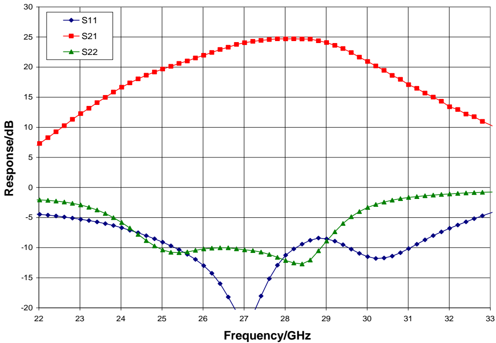
Narrow-band Performance, V_{dd} = 28\text{ V} , V_{gg1, 2, 3} = -4\text{ V} , I_{dd} = 350\text{ mA} , T_A = 25\text{ °C}
