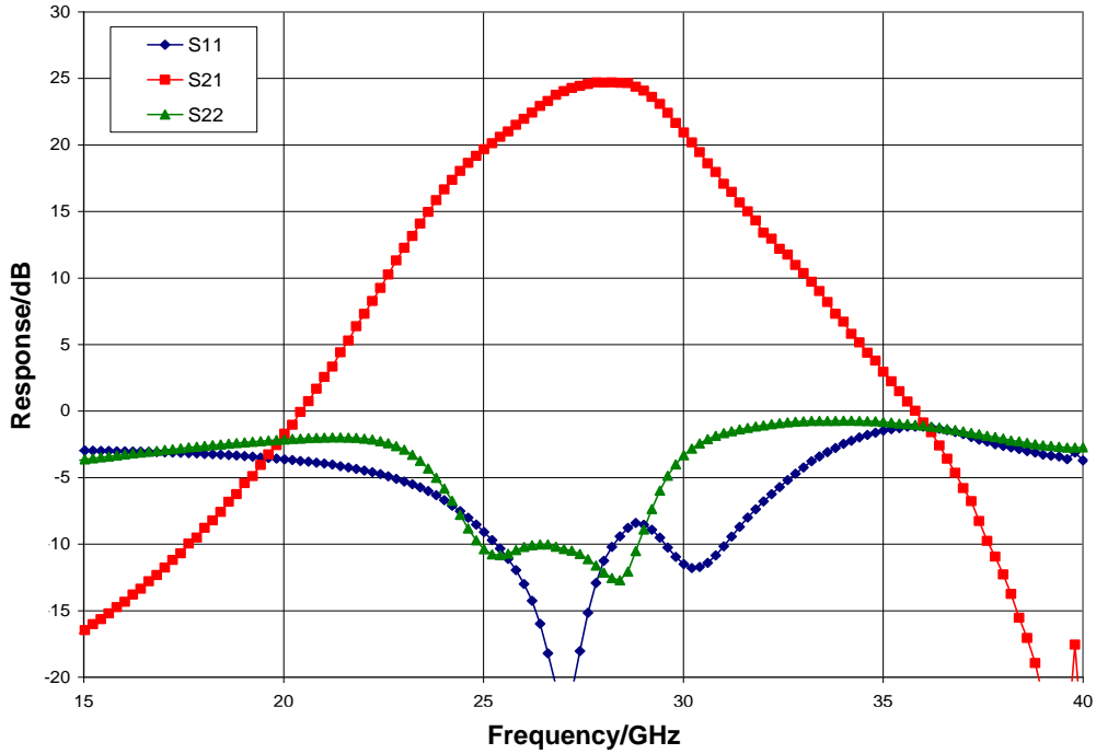
Broadband Performance, V_{dd} = 28\text{ V} , V_{gg1, 2, 3} = -4\text{ V} , I_{dd} = 350\text{ mA} , T_A = 25\text{ °C}
