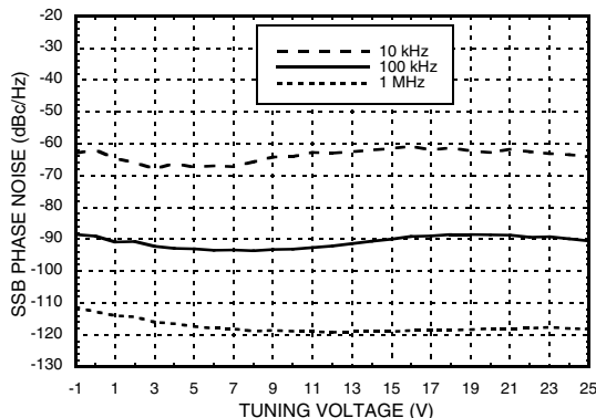
SSB Phase Noise vs. Tuning Voltage, T = +25\text{ }^{\circ}C
