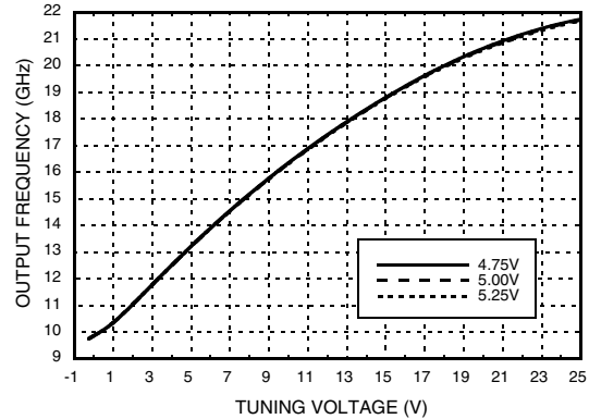
Frequency vs. Tuning Voltage, T = +25\text{ }^{\circ}C
