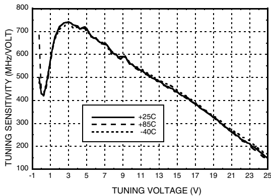
Sensitivity vs. Tuning Voltage, V_{cc} = +5V, T = +25\text{ }^{\circ}C
