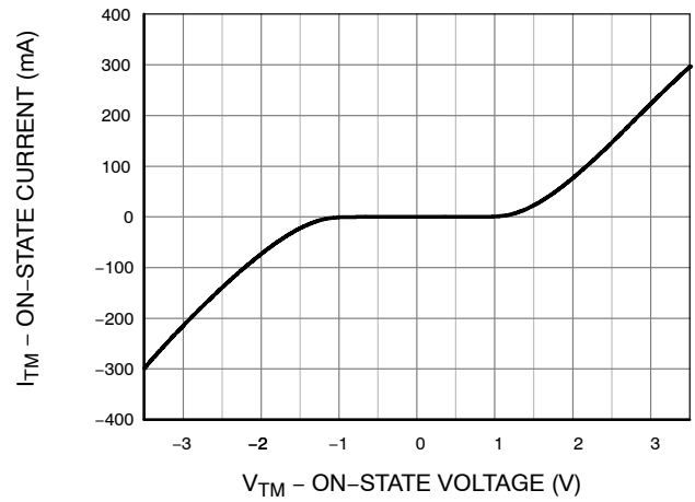
Figure 2. On-State Characteristics
