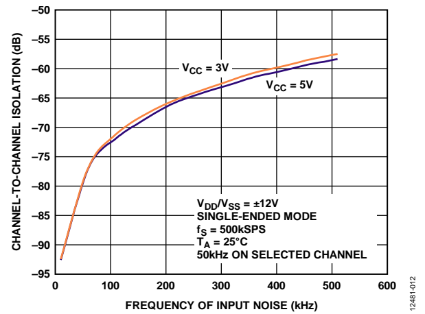
Figure 14. Channel-to-Channel Isolation
