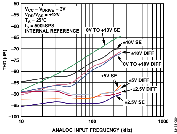
Figure 10. THD vs. Analog Input Frequency for Single-Ended (SE) and True Differential (Diff) Mode at 3 V V_{CC}
