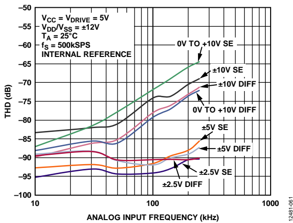
Figure 11. THD vs. Analog Input Frequency for Single-Ended (SE) and True Differential (Diff) Mode at 5 V V_{CC}
