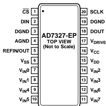
Figure 3. Pin Configuration
