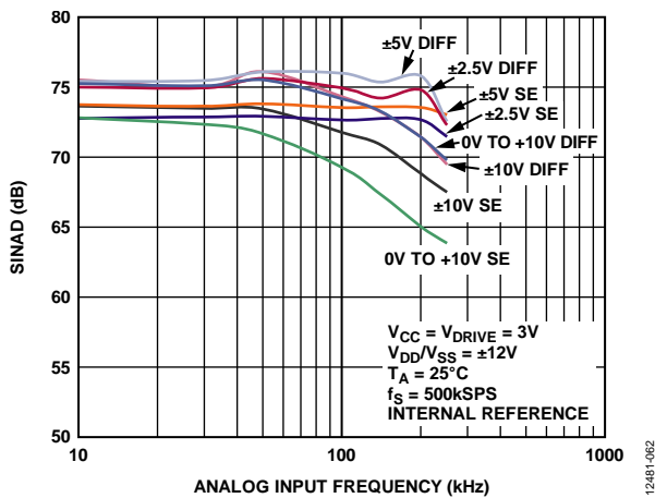
Figure 12. SINAD vs. Analog Input Frequency for Single-Ended (SE) and True Differential (Diff) Mode at 3 V V_{CC}
