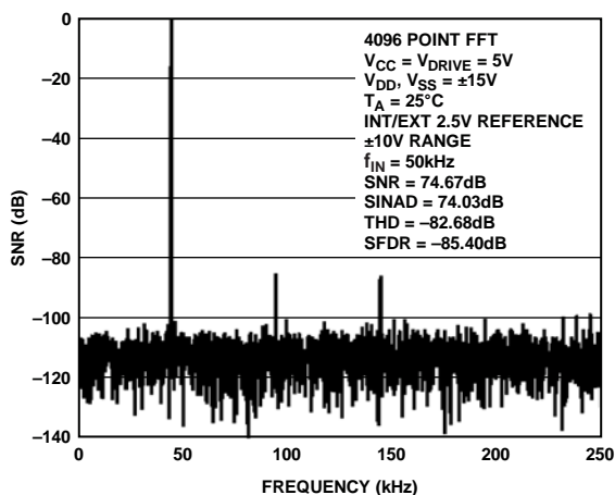
Figure 5. FFT Single-Ended Mode
