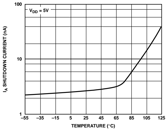
Figure 34. Shutdown Current vs. Temperature
