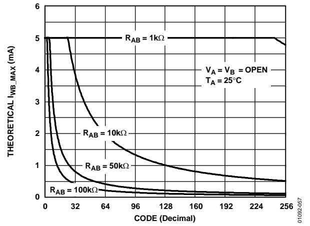
Figure 36. I_{WB\_MAX} vs. Code
