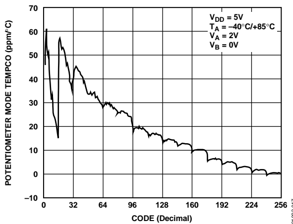
Figure 17. \Delta V_{WB}/\Delta T Potentiometer Mode Tempo
