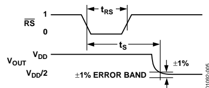
Figure 5. Reset Timing Diagram
