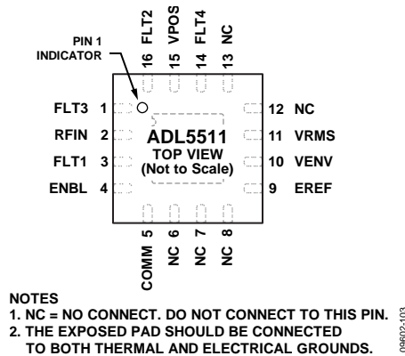
Figure 3. Pin Configuration
