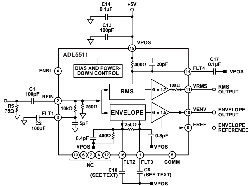
Figure 49. Basic Connections
