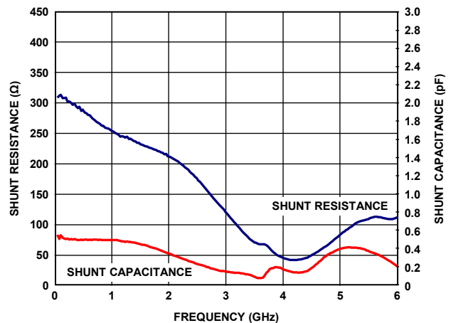
Figure 9. Input Impedance vs. Frequency
