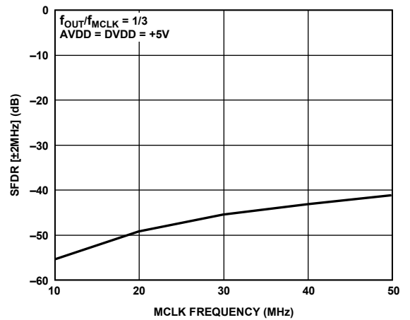
Figure 10. Wideband SFDR vs. MCLK Frequency
