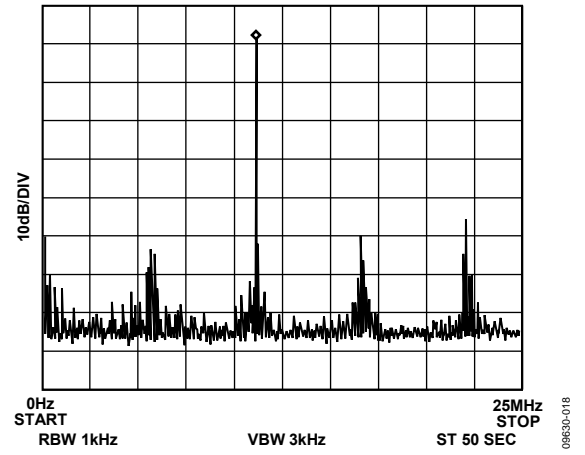
Figure 18. f_{MCLK} = 50 \text{ MHz} , f_{OUT} = 11.1 \text{ MHz} . Frequency Word = 38D4DF4
