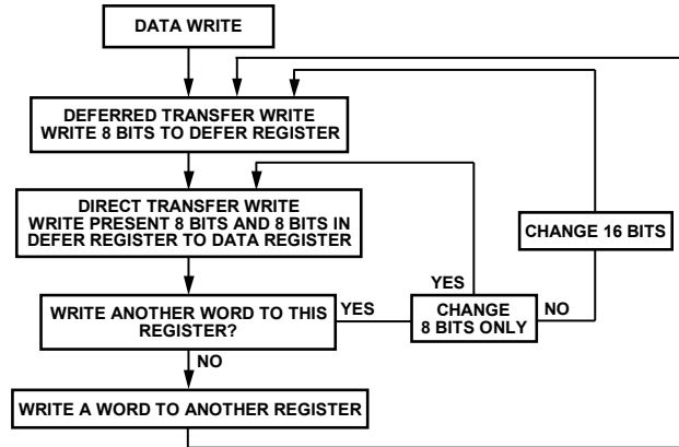
Figure 24. Data Writes
