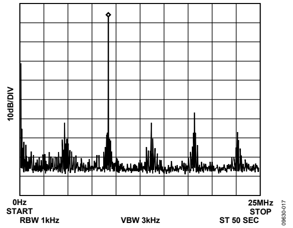
Figure 17. f_{MCLK} = 50 \text{ MHz} , f_{OUT} = 9.1 \text{ MHz} . Frequency Word = 2E978D00
