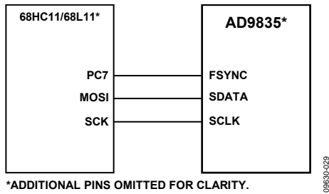
*ADDITIONAL PINS OMITTED FOR CLARITY. Figure 27. 68HC11/68L11-to-AD9835 Interface
