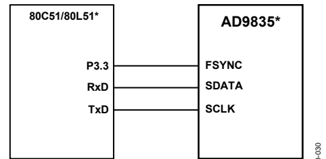
*ADDITIONAL PINS OMITTED FOR CLARITY. Figure 28. 80C51/80L51 to AD9835 Interface
