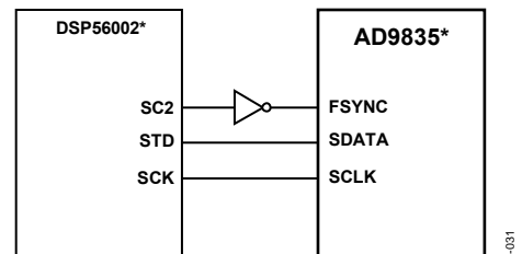
*ADDITIONAL PINS OMITTED FOR CLARITY. Figure 29. AD9835-to-DSP56002 Interface
