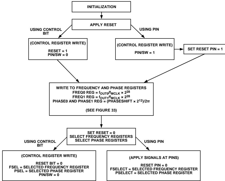
Figure 32. Initialization
