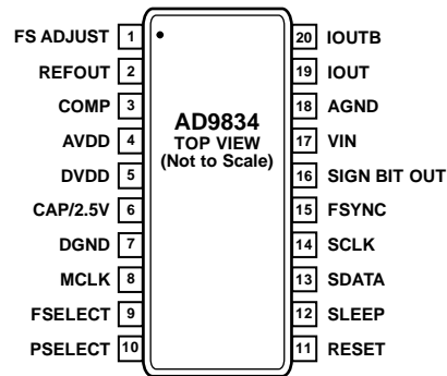
Figure 6. Pin Configuration
