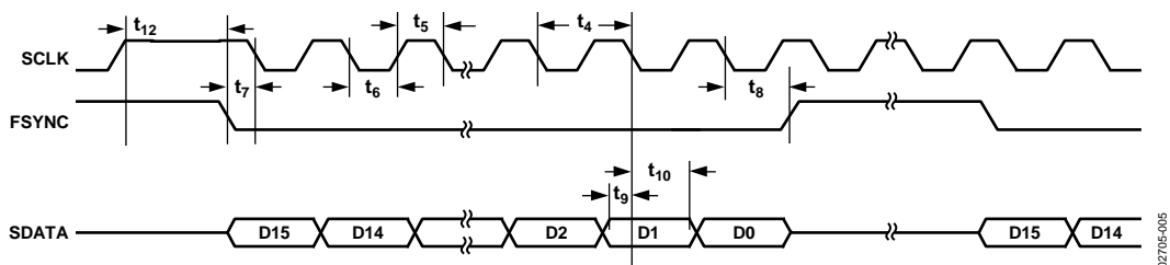
Figure 5. Serial Timing
