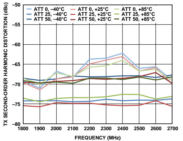
Figure 48. TX Second-Order Harmonic Distortion (HD2) vs. Frequency
