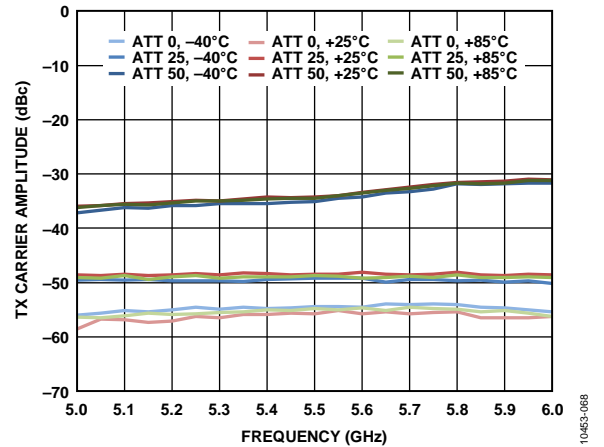
Figure 68. TX Carrier Rejection vs. Frequency
