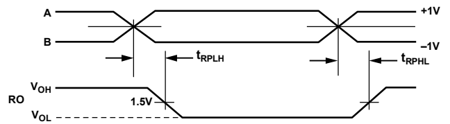
Figure 21. Receiver Propagation Delays
