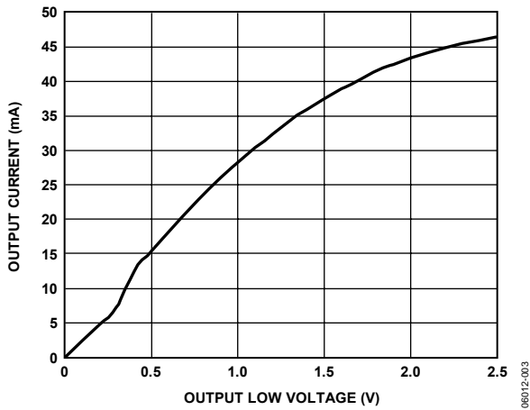
Figure 3. Output Current vs. Receiver Output Low Voltage
