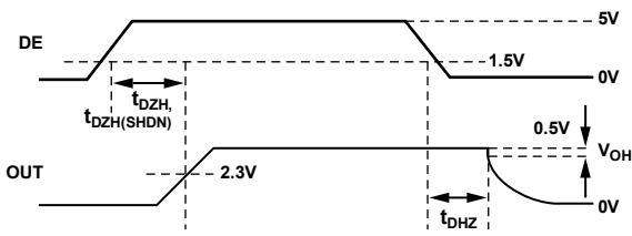
Figure 18. Driver Enable and Disable Times ( t_{DZH} , t_{DZH} , t_{DZH(SHDN)} )
