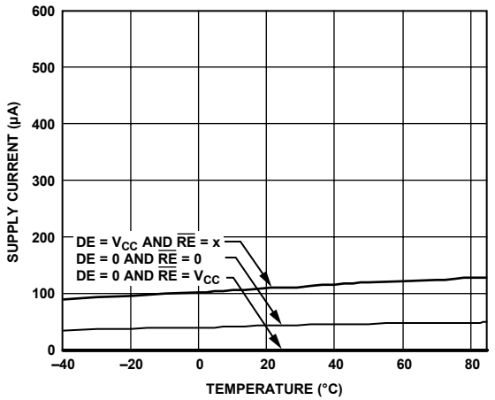
Figure 11. ADM483E Supply Current vs. Temperature
