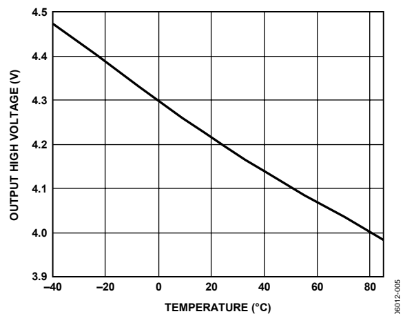
Figure 5. Receiver Output High Voltage vs. Temperature
