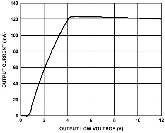
Figure 9. Output Current vs. Driver Output Low Voltage
