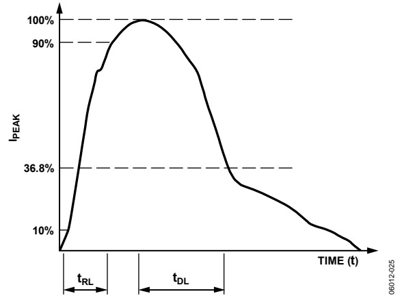
Figure 25. Human Body Model ESD Current Waveform
