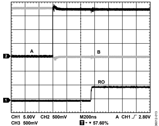
Figure 13. ADM483E Receiver t_{PHL}
