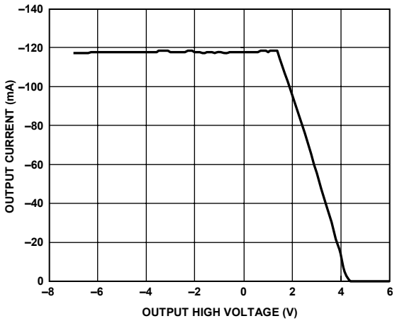
Figure 10. Output Current vs. Driver Output High Voltage
