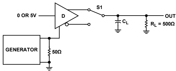
Figure 17. Driver Propagation Delays
